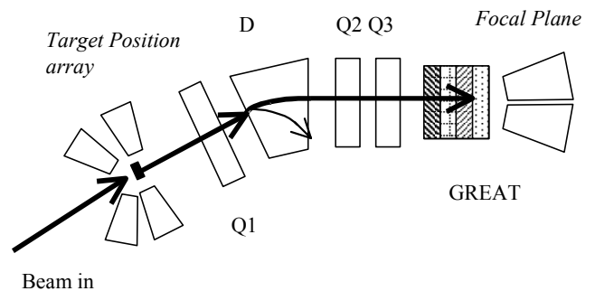
Figure 1: GREAT with a recoil separator and target array
