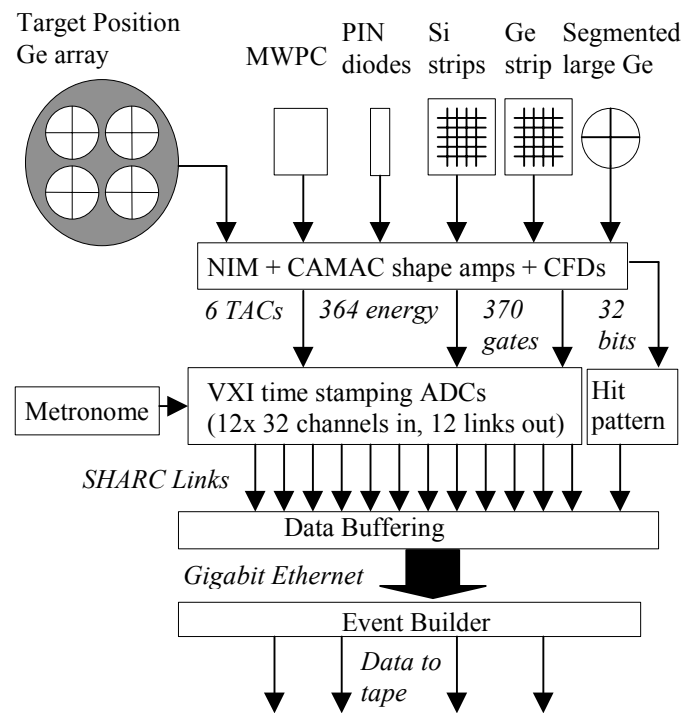
Figure 2 GREAT TDR System Diagram
