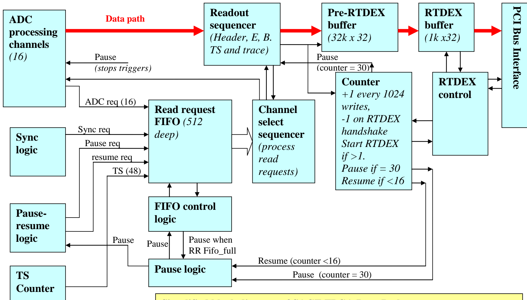
Simplified block diagram of SAGE FPGA Data Path (firmware rev 4.x Date 25-03-10)
